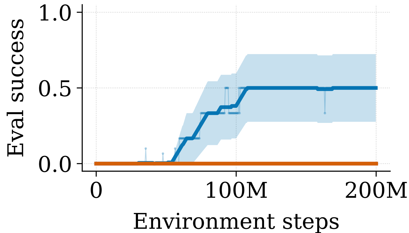
Maximum overhang 5 · eval (roll. mean w=21 )
